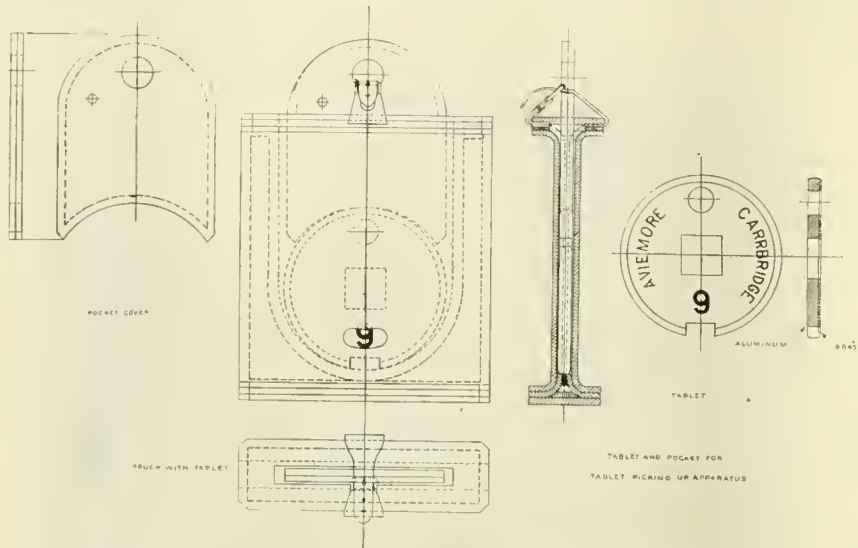
FIG. 3.—LEATHER POUCH AND TABLET USED ON THE HIGHLAND RAILWAY OF SCOTLAND.
